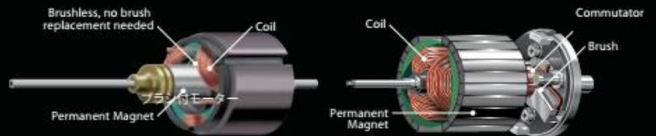
● Brushless Motor
